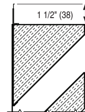
OPT. FLANGED FRAME
